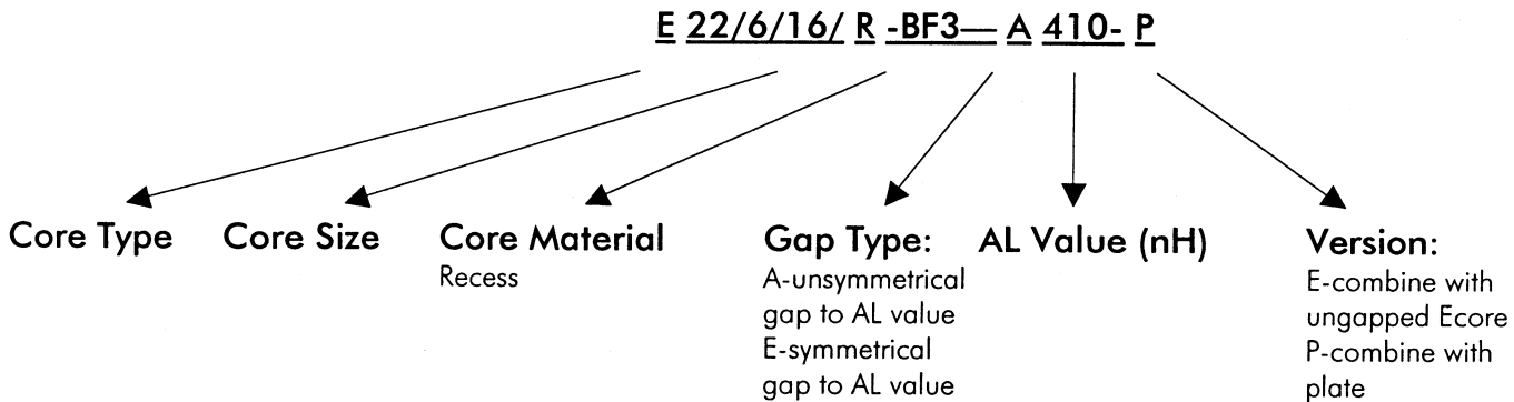
Type number structure for cores
