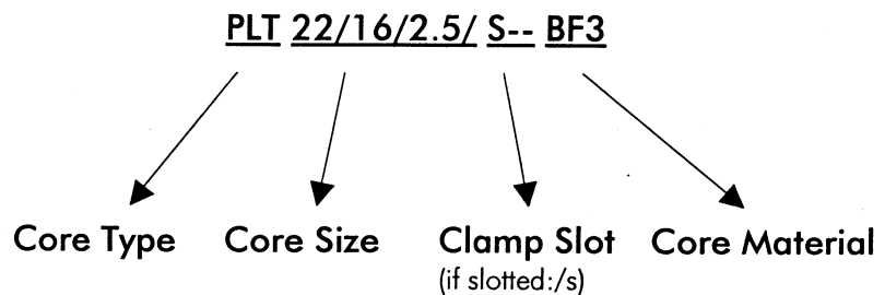
Type number structure for plates
